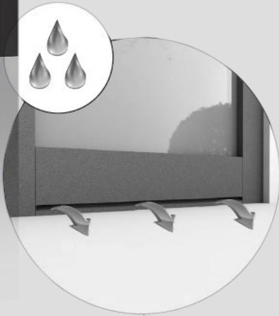
Concealed drainage system in sidelight.
